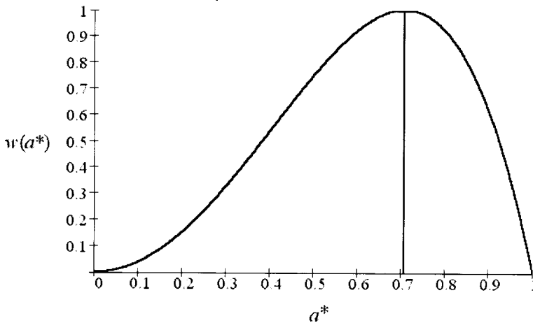
Figure 2 Cureton-Mulaik Weight Function. m = 2 \quad m^{-1/2} = .71
