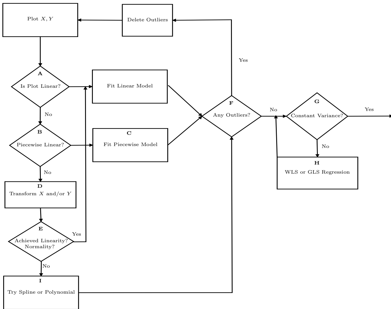
Figure 1: Steps in Bivariate Continuous Regression
